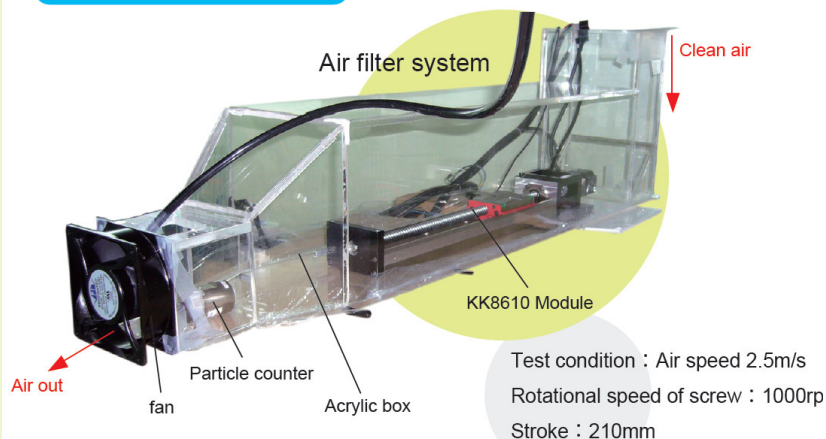
Dust generation test of grease
